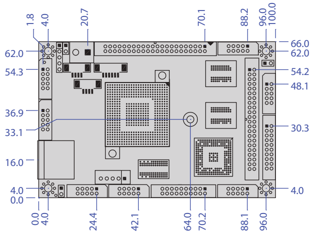
Unit: mm
